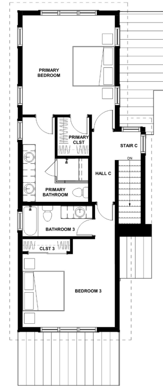
4. UPPER LEVEL - MRKG A2.4 1/4" = 1'-0"
