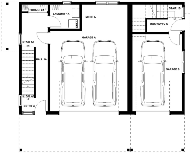
2 GROUND LEVEL - MRKG A2.4 / 1/4" = 1'-0"
